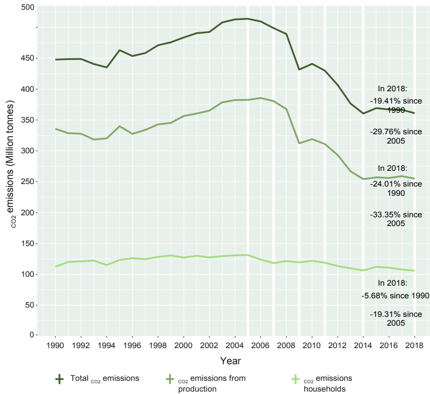
Figure 19 - CO 2 emissions by households and production activities
